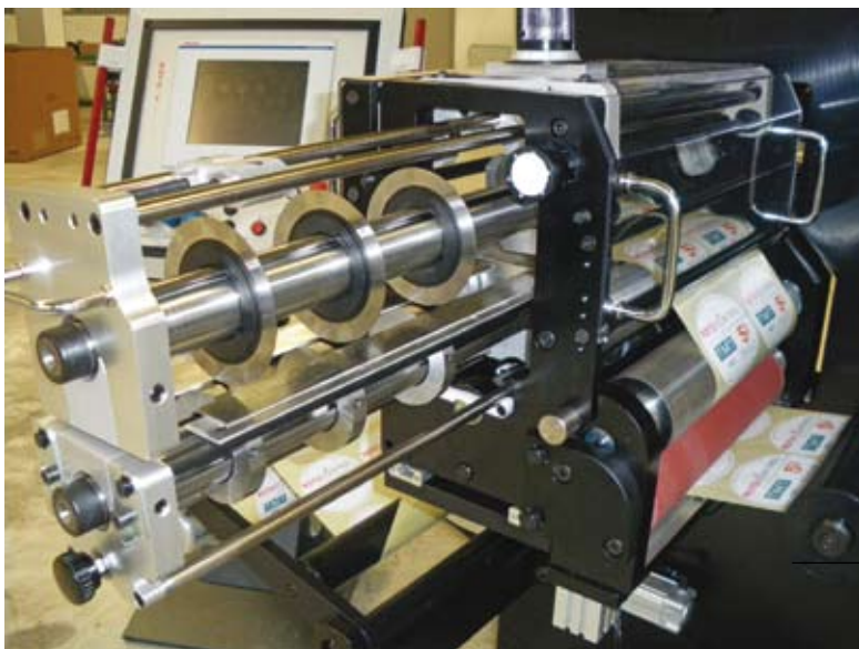
A RotoControl RSP single pass 100% security inspection machine has been installed at Advanced Labels in Durban.
